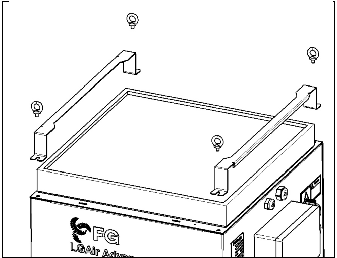
Fig. 9: Removing retaining bracket
