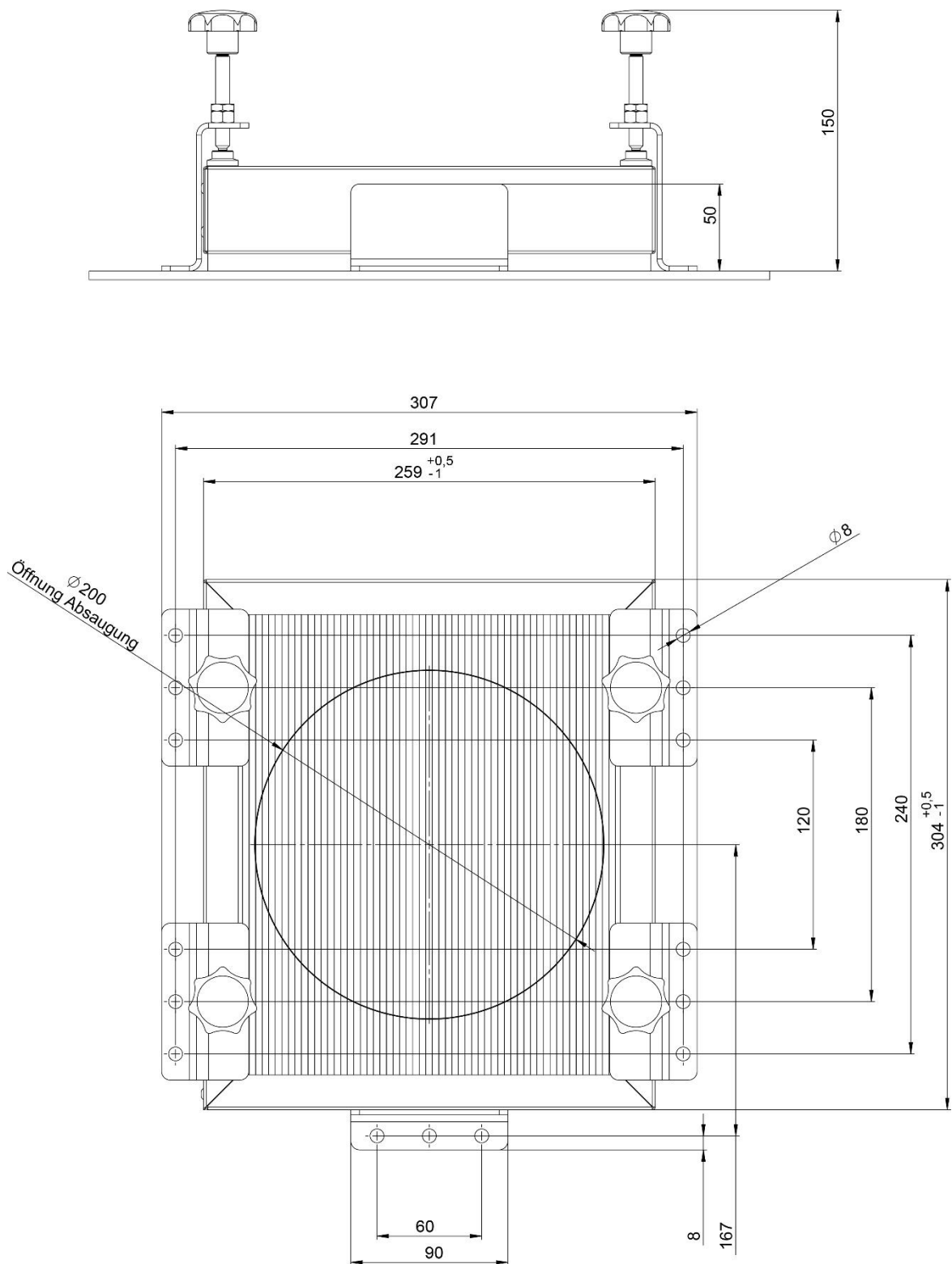
Fig. 16: Installing a Miofilter panel in the machine tool
