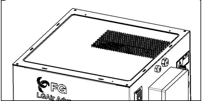
Fig. 10: Removing the HEPA filter and replacing it with a new original element
