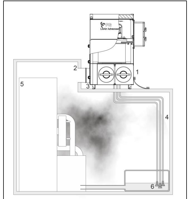
Fig. 4: Installing the oil mist separator
