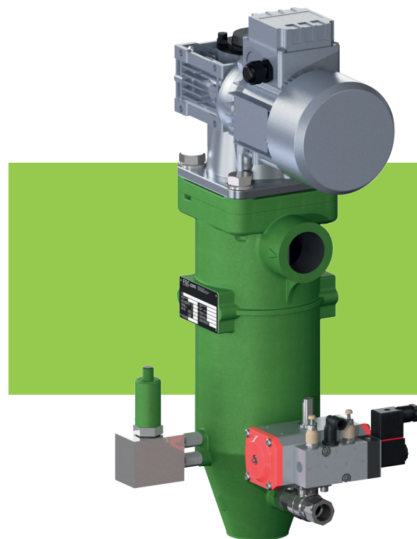
AF 122 with PIS3310 IO-Link and gear motor
