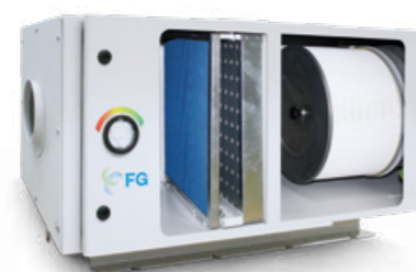
ASL aerosol separator device for emulsion mist
